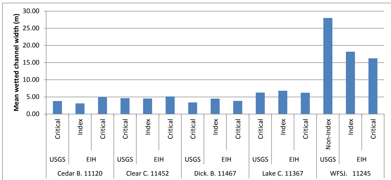
Figure 15. Mean wetted channel width (m) recorded at five field survey sites by EIH and USGS. Corresponds to data in Table 4.
