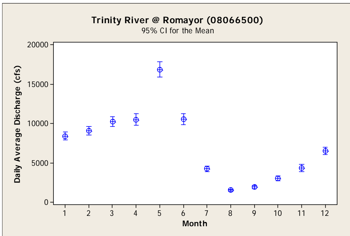
Figure 35. Monthly mean and 95% confidence intervals for daily average flow recorded at the USGS Trinity River at Romayor (08066500) gage from 1925 through 2008.
