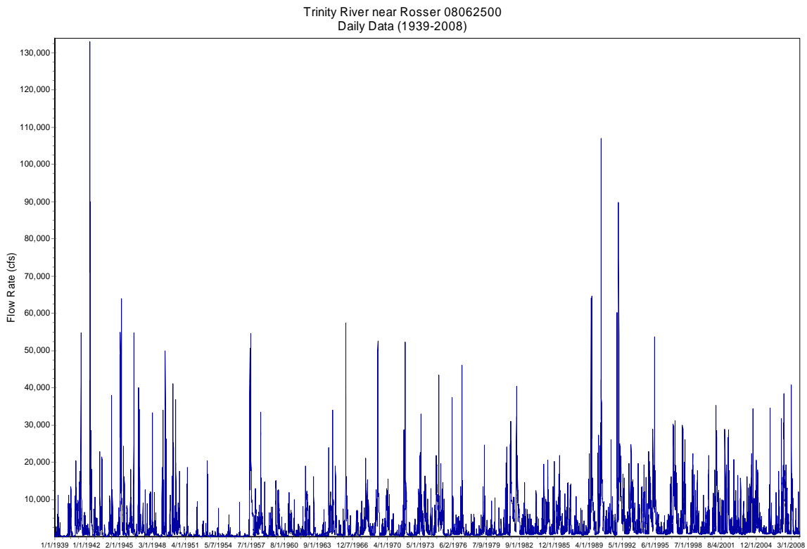
Figure 18. Average daily flows recorded at the USGS Trinity River at Rosser (08062500) gage from 1939 through 2008.
