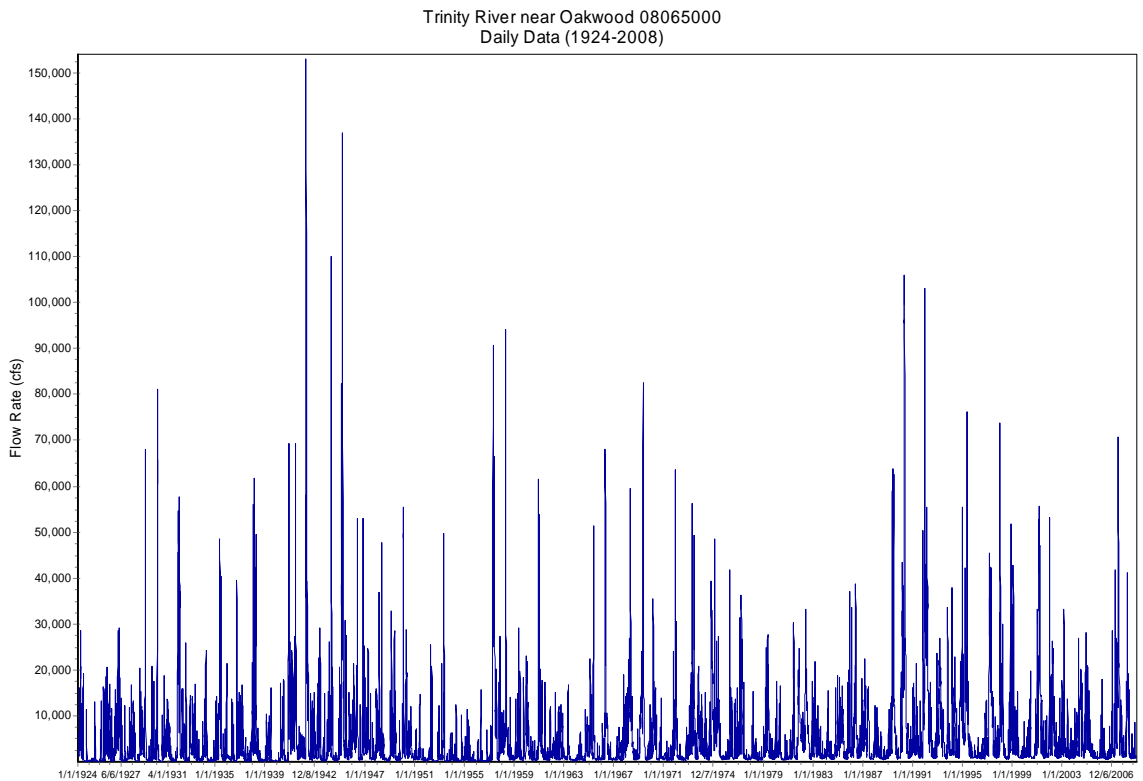
Figure 26. Average daily flows recorded at the USGS Trinity River near Oakwood (08065000) gage from 1924 through 2008.
