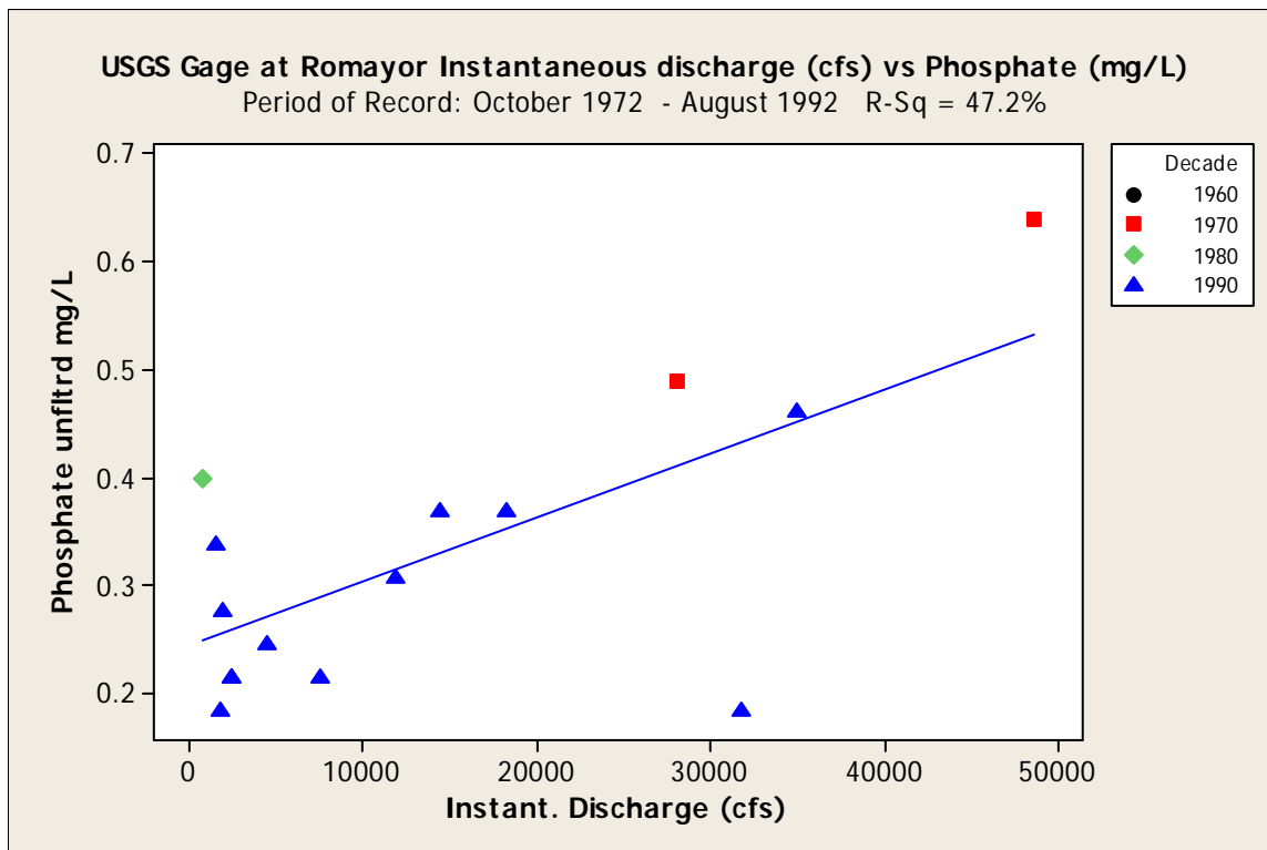
Figure 127. Flow versus total unfiltered phosphate at the Trinity River at Romayor 08066500 gage during 1972 through 1992. Matching flow and phosphate data lacking for 1960s and 2000s.
