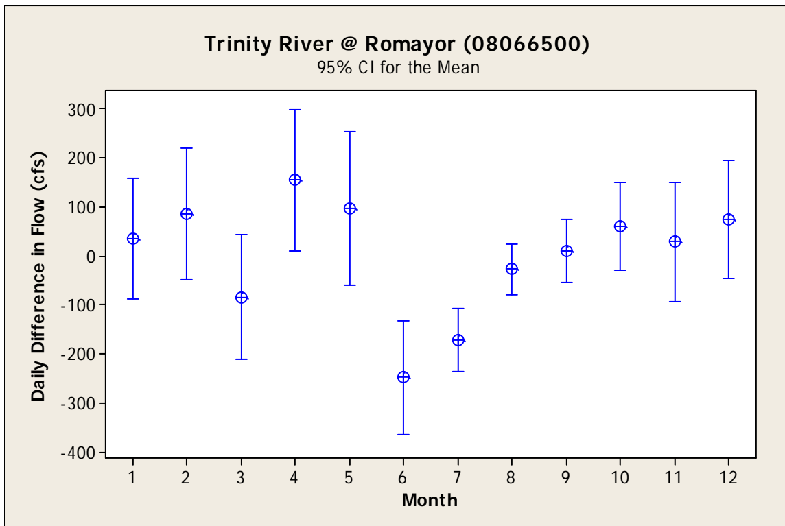
Figure 37. Monthly mean and 95% confidence intervals for daily difference in average daily flows between successive dates recorded at the USGS Trinity River at Romayor (08066500) gage from 1925 through 2008.
