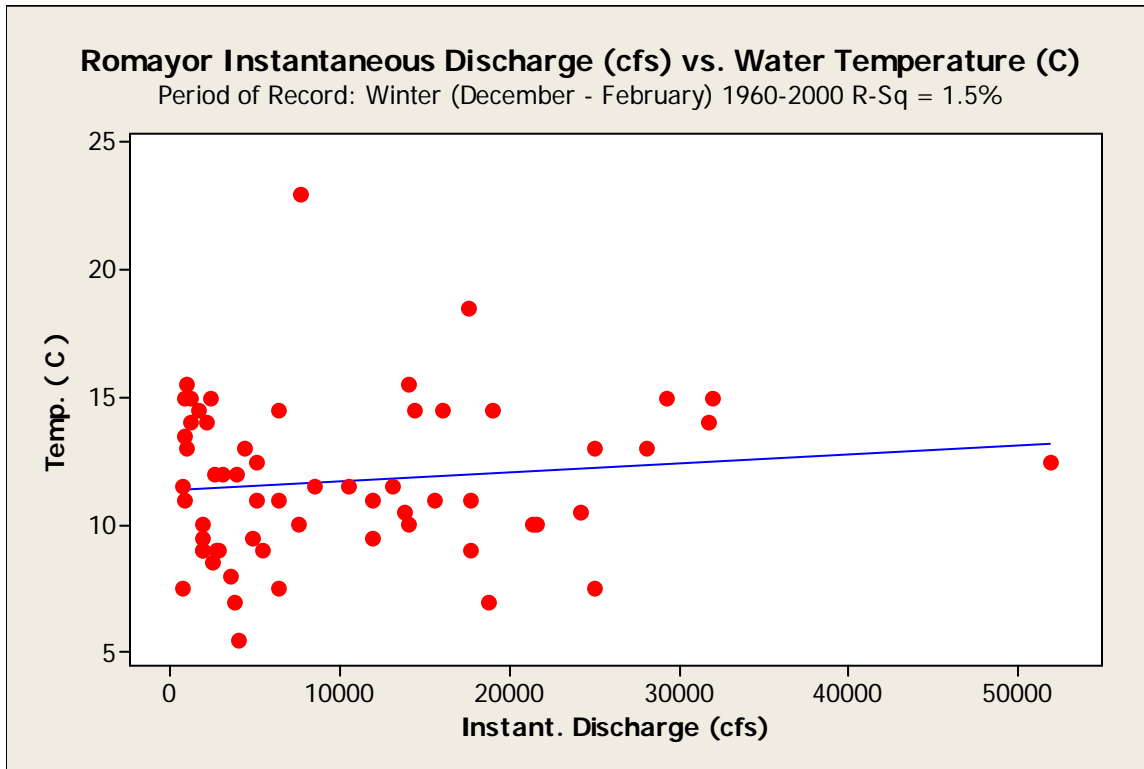
Figure 114. Flow versus winter water temperature at the Trinity River at Romayor 08066500 gage during 1960 through 1995.
