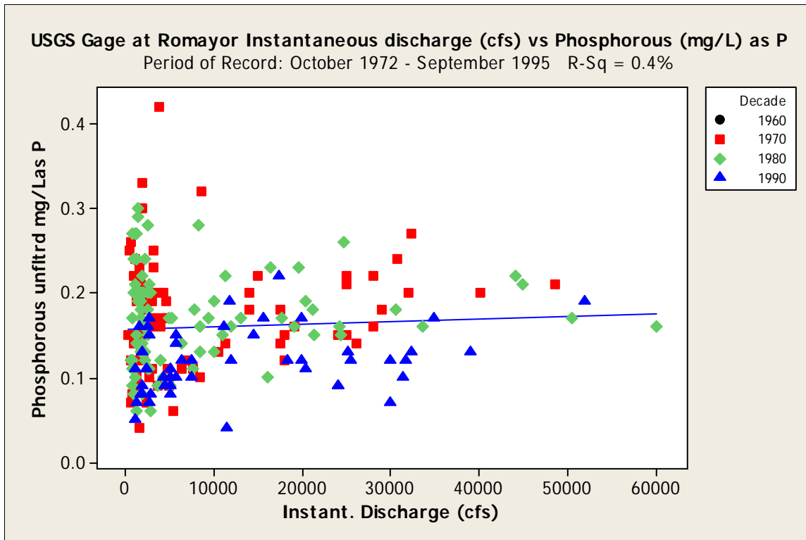
Figure 128. Flow versus total unfiltered phosphorus at the Trinity River at Romayor 08066500 gage during 1972 through 1995. Matching flow and phosphate data lacking for 1960s and 2000s.
