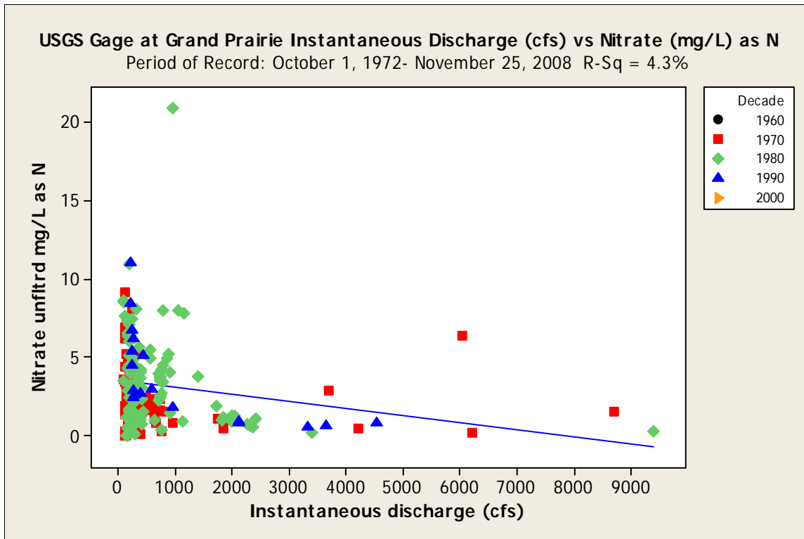
Figure 54. Flow versus nitrate at the West Fork Trinity River at Grand Prairie 08049500 gage during 1972 through 2008. Matching flow and nitrate data lacking for 1960s and 2000s.
