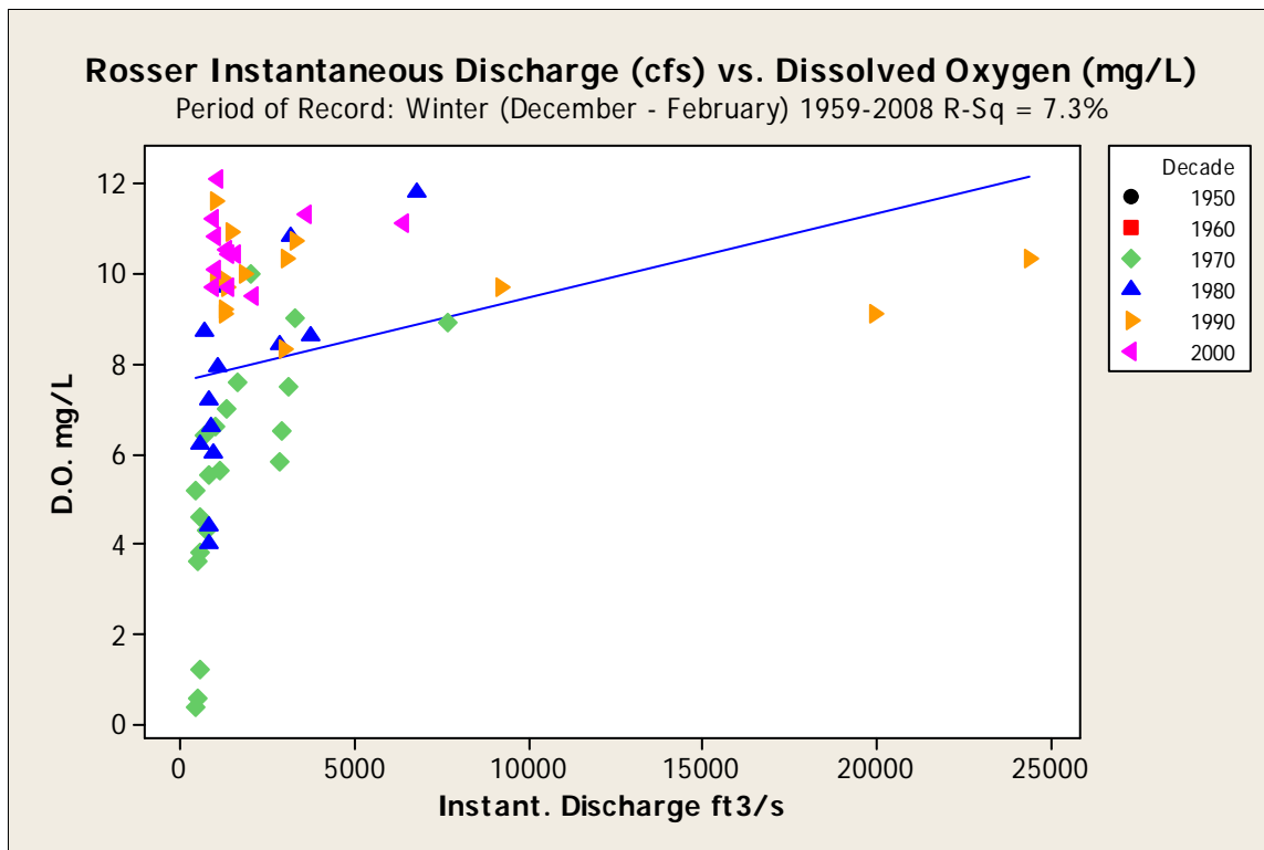
Figure 63. Flow versus winter dissolved oxygen at the Trinity River at Rosser 08062500 gage during 1959 through 2008. Matching flow and dissolved oxygen data lacking for 1960s.
