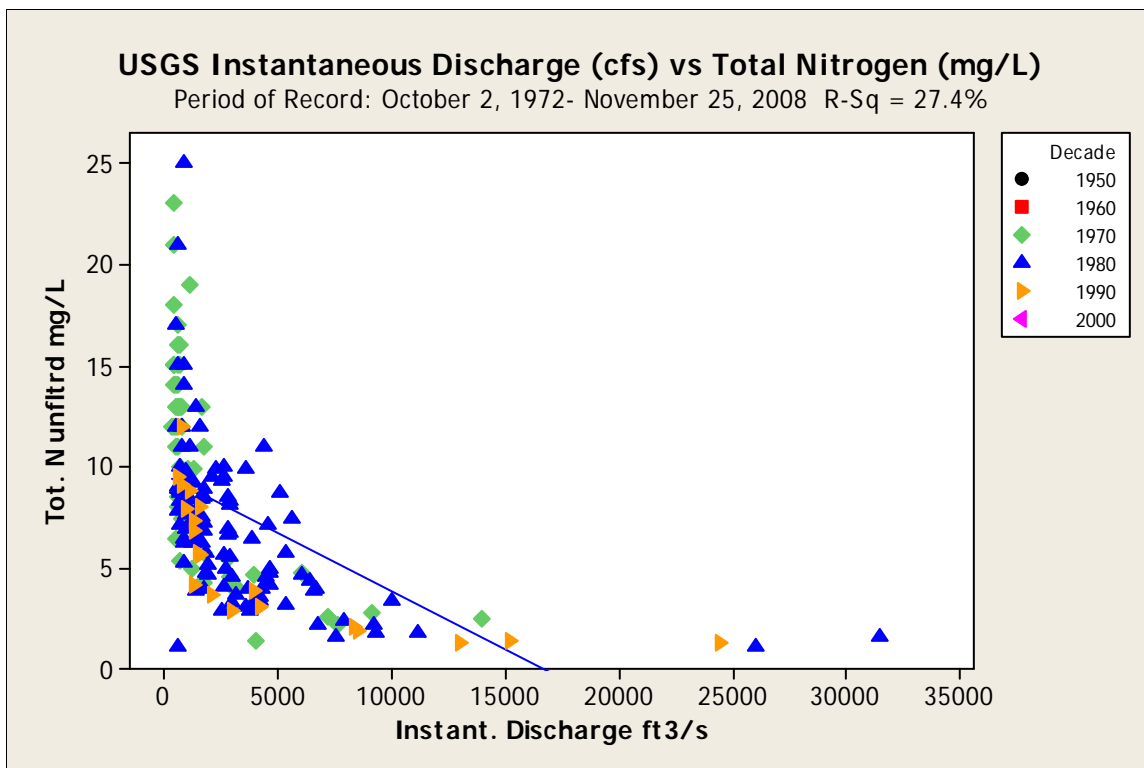
Figure 68. Flow versus total nitrogen (unfiltered) at the Trinity River at Rosser 08062500 gages during 1972 through 2008. Matching flow and total nitrogen data lacking for 1950s, 1960s and 2000s.
