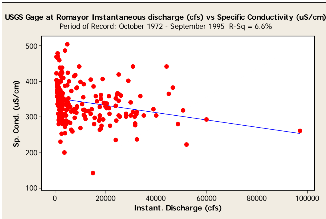
Figure 122. Flow versus specific conductance at the Trinity River at Romayor 08066500 gage during 1972 through 1995.
