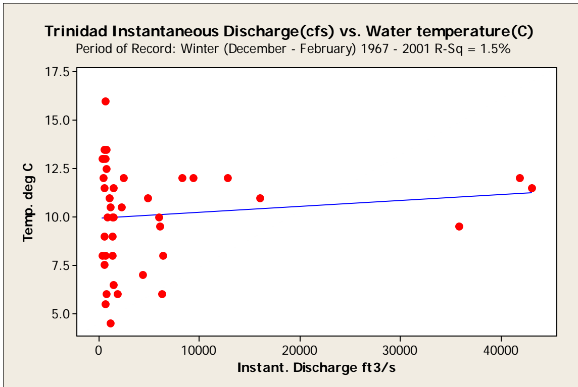
Figure 75. Flow versus winter water temperature at the Trinity River at Trinidad 08062700 gage during 1967 through 2001.
