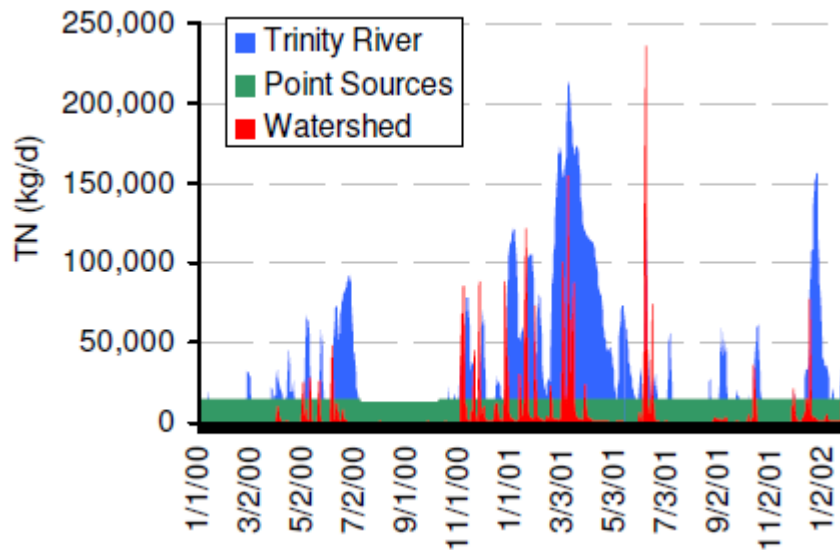
Figure 137. Total nitrogen loads estimated presented and cited by (Jensen et al. 2003). Original source: (Clingenpeel 2002)
