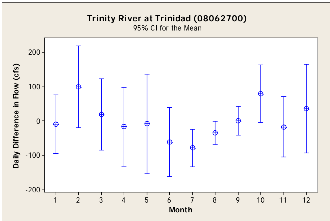
Figure 25. Monthly mean and 95% confidence intervals for daily difference in average daily flows between successive dates recorded at the USGS Trinity River at Trinidad (08062700) gage from 1965 through 2008.
