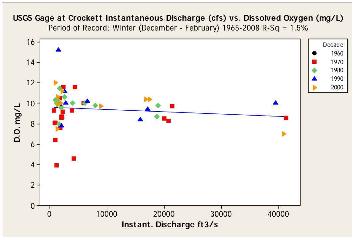
Figure 97. Flow versus winter dissolved oxygen at the Trinity River near Crockett 08065350 gage during 1965 through 2008. Matching flow and dissolved oxygen data lacking for 1960s.
