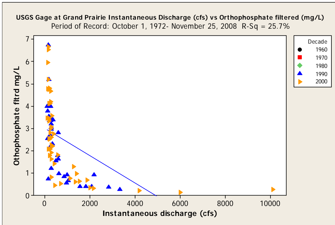
Figure 58. Flow versus orthophosphate at the West Fork Trinity River at Grand Prairie 08049500 gage during 1972 through 2008. Matching flow and phosphorus data lacking for 1960s through 1980s.
