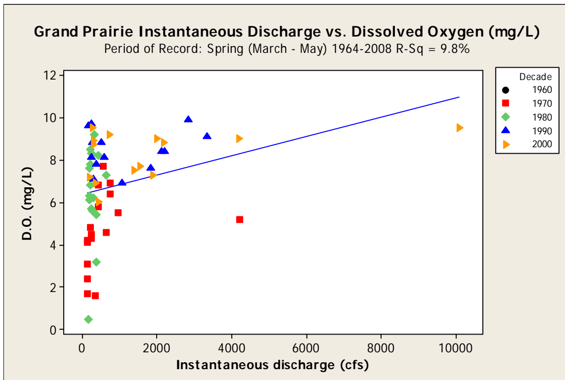
Figure 48. Flow versus spring dissolved oxygen at the West Fork Trinity River at Grand Prairie 08049500 gage during 1964 through 2008. Matching flow and dissolved oxygen data lacking for 1960s.
