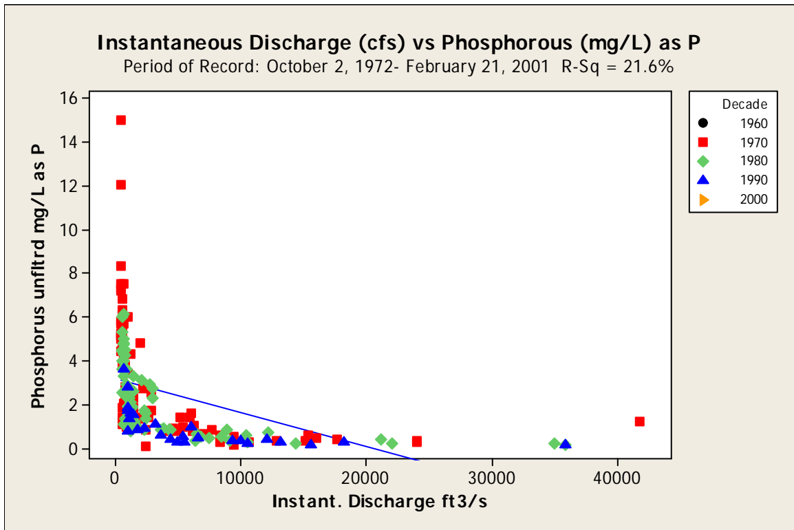
Figure 88. Flow versus total unfiltered phosphorus at the Trinity River at Trinidad 08062700 gage during 1972 through 2001. Matching flow and total phosphorus data lacking for 1960s and 2000s.
