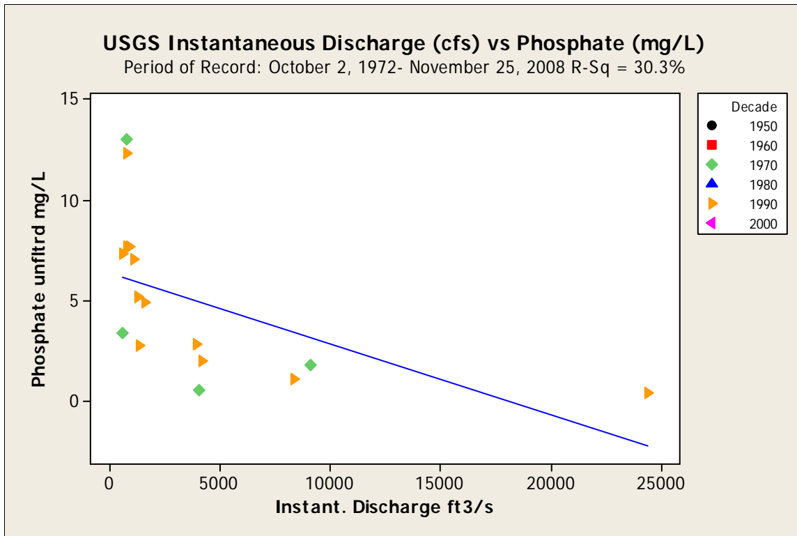
Figure 73. Flow versus total phosphate unfiltered at the Trinity River at Rosser 08062500 gage during 1972 through 2008. Matching total phosphate and flow data lacking for 1950s, 1960s, 1980s, and 2000s.
