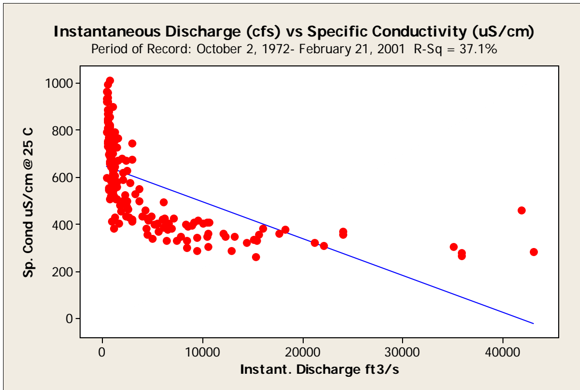
Figure 83. Flow versus specific conductance at the Trinity River at Trinidad 08062700 gage during 1972 through 2001.
