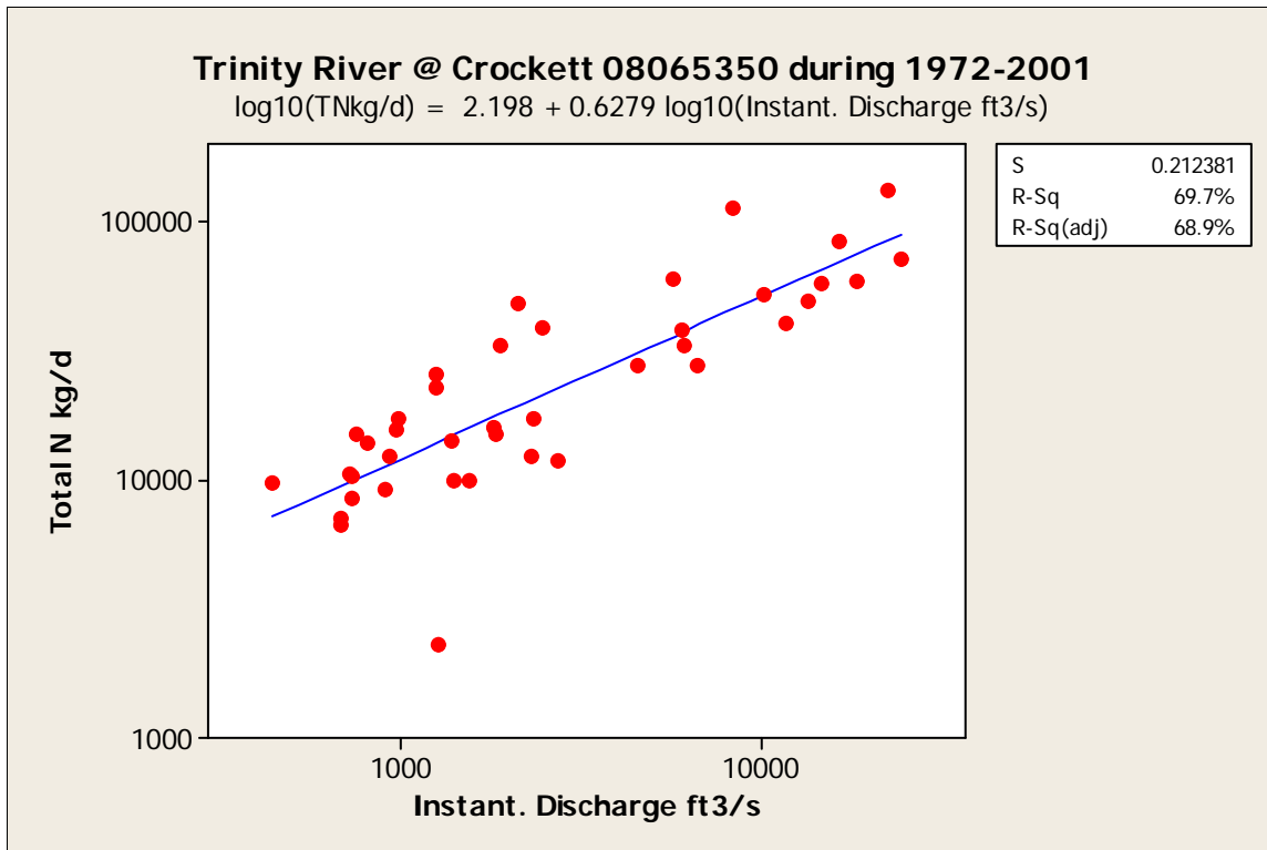
Figure 109. Flow versus total nitrogen loading at the Trinity River at Crockett 08065350 gage during 1972 through 2001.
