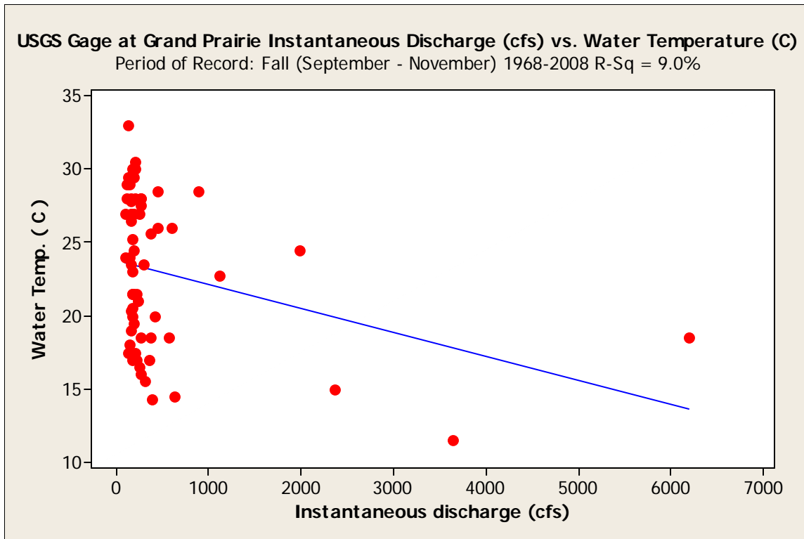
Figure 46. Flow versus fall water temperature at the West Fork Trinity River at Grand Prairie 08049500 gage during 1968 through 2008.
