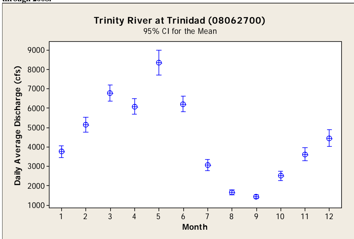
Figure 23. Monthly mean and 95% confidence intervals for daily average flow recorded at the USGS Trinity River at Trinidad (08062700) gage from 1965 through 2008.
