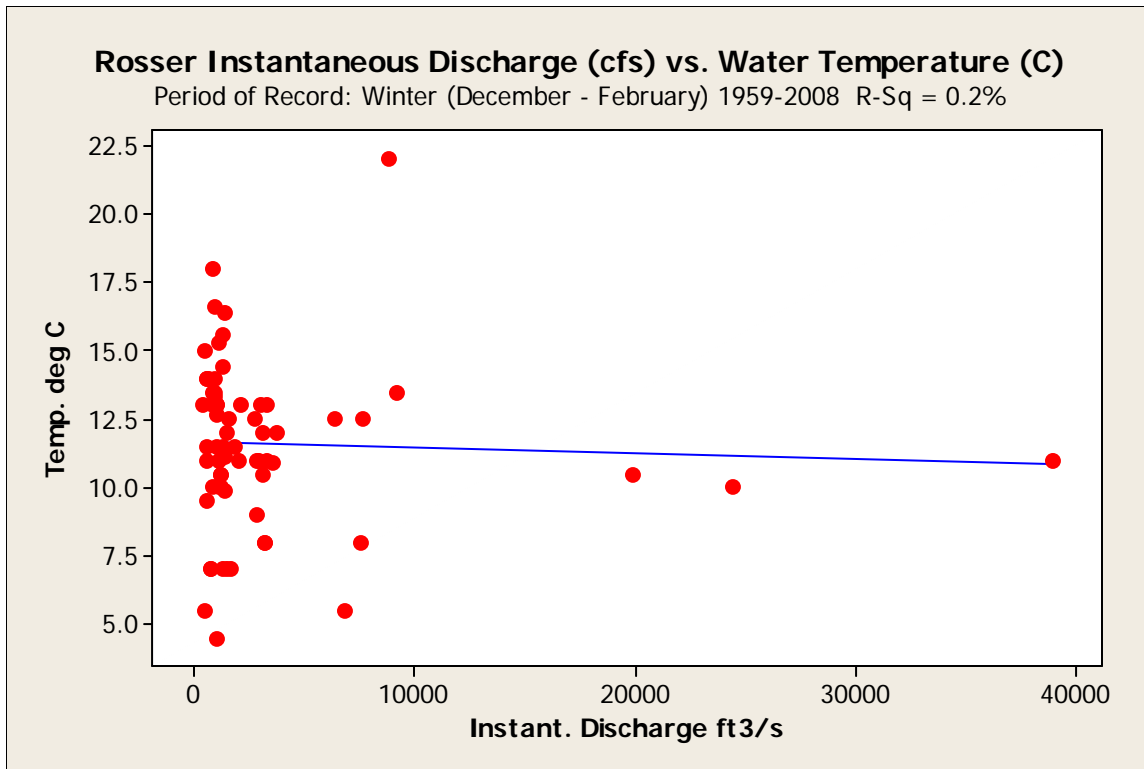
Figure 59. Flow versus winter temperature at the Trinity River at Rosser 08062500 gage during 1959 through 2008.
