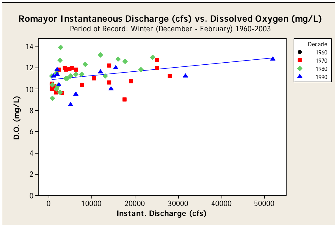
Figure 118. Flow versus winter dissolved oxygen at the Trinity River at Romayor 08066500 gage during 1960 through 2003. Matching flow and dissolved oxygen data lacking for 1960s and 2000s.
