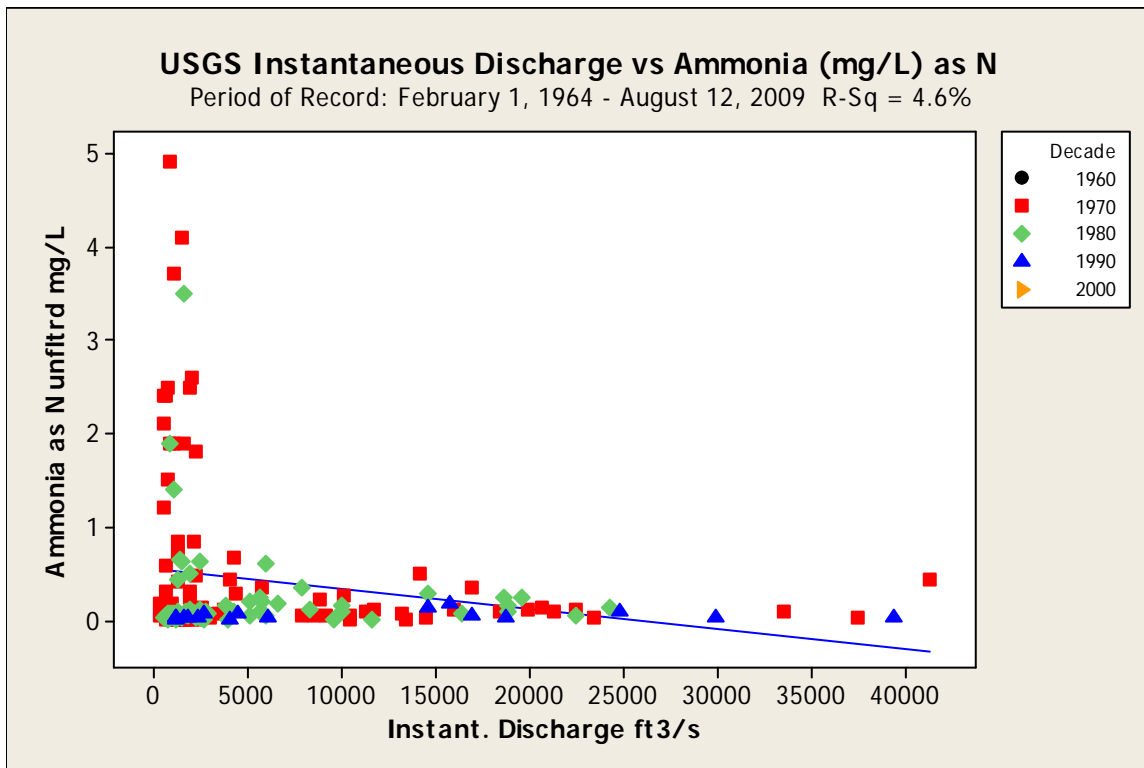
Figure 104. Flow versus unfiltered ammonia as nitrogen concentration at the Trinity River near Crockett 08065350 gage during 1972 through 2001. Matching flow and ammonia nitrogen data lacking for 1960s and 2000s.
