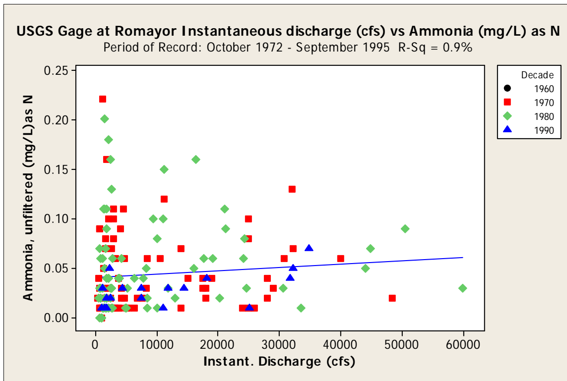
Figure 124. Flow versus ammonia nitrogen at the Trinity River at Romayor 08066500 gage during 1972 through 1995. Matching flow and total nitrogen data lacking for 1960s and 2000s.
