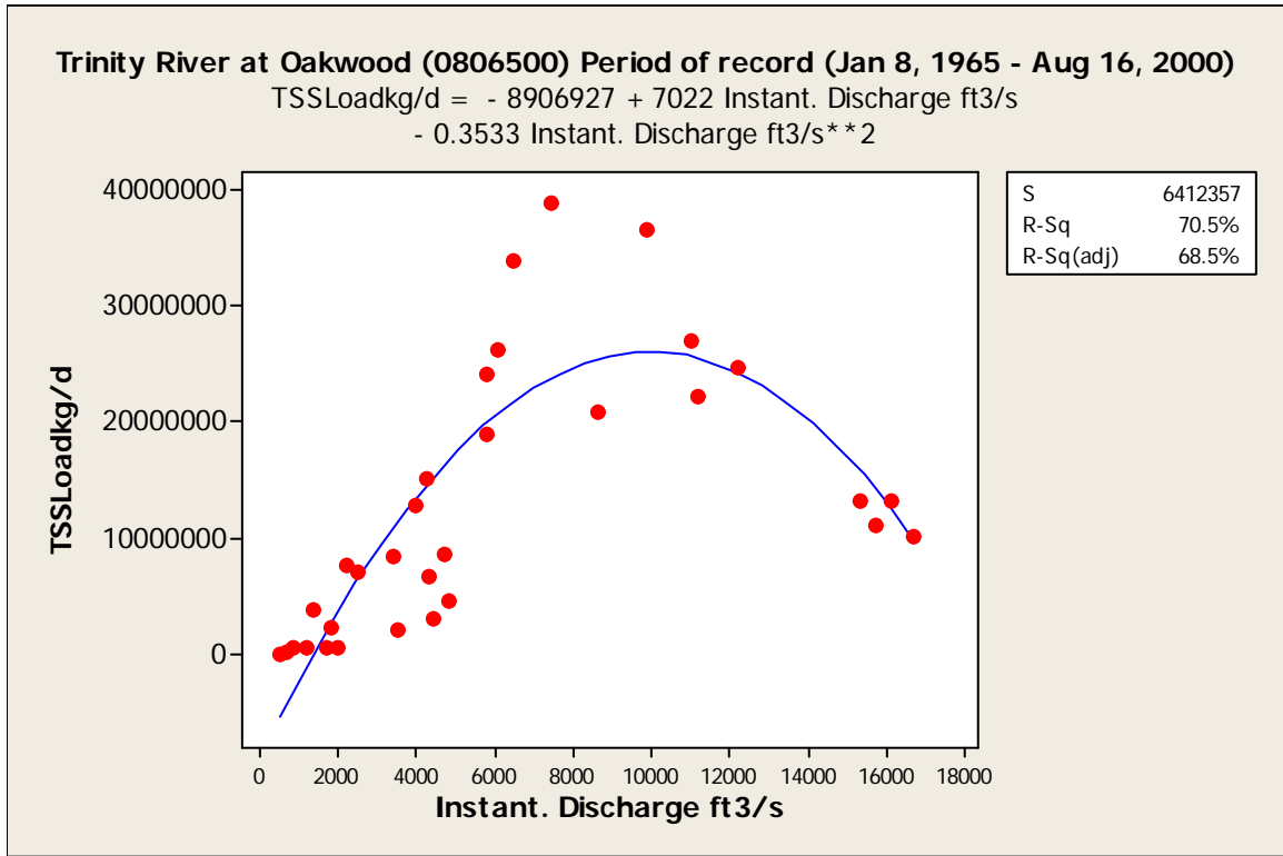
Figure 92. Flow versus suspended sediment load at the Trinity River near Oakwood 08065000 gage during 1965 through 2000. Paired flow and suspended solids data lacking from 1960s, 1980s and 2000s.
