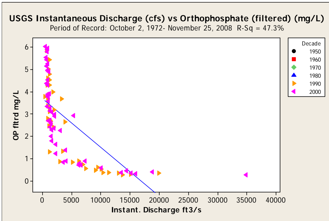
Figure 74. Flow versus filtered orthophosphate at the Trinity River at Rosser 08062500 gage during 1972 through 2008. Matching orthophosphate and flow data available for 1990s, and 2000s only.
