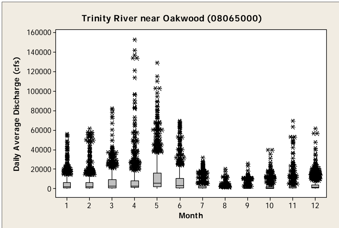
Figure 28. Monthly median, interquartile range (boxes), extended range (1.5 X quartile = line) and outliers (*) for daily average flows recorded at the USGS Trinity near Oakwood (08065000) gage from 1924 through 2008.
