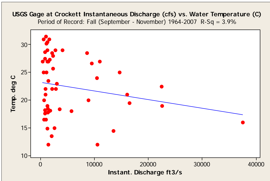
Figure 96. Flow versus fall water temperature at the Trinity River near Crockett 08065350 gage during 1964 through 2007.
