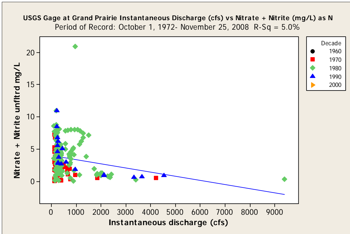
Figure 55. Flow versus nitrate+nitrite at the West Fork Trinity River at Grand Prairie 08049500 gage during 1972 through 2008. Matching flow and nitrate + nitrite data lacking for 1960s and 2000s.
