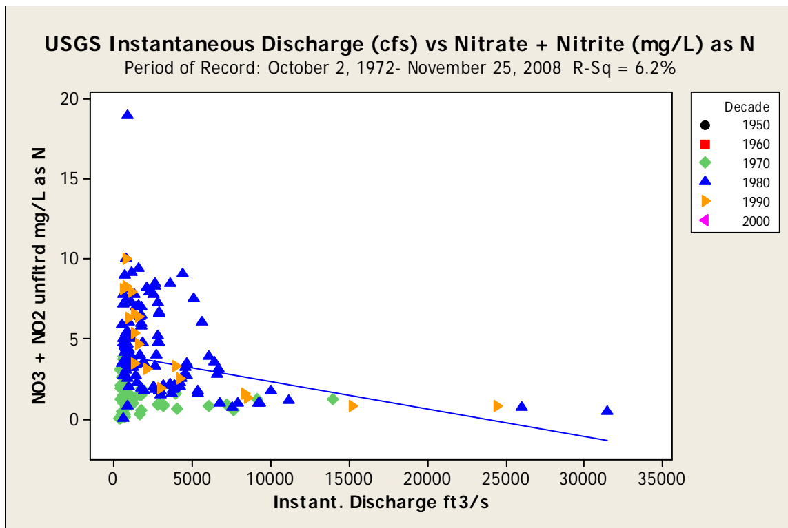
Figure 69. Flow versus nitrate + nitrite as N at the Trinity River at Rosser 08062500 gage during 1972 through 2008. Matching flow and nitrates + nitrites data lacking for 1950s, 1960s and 2000s.
