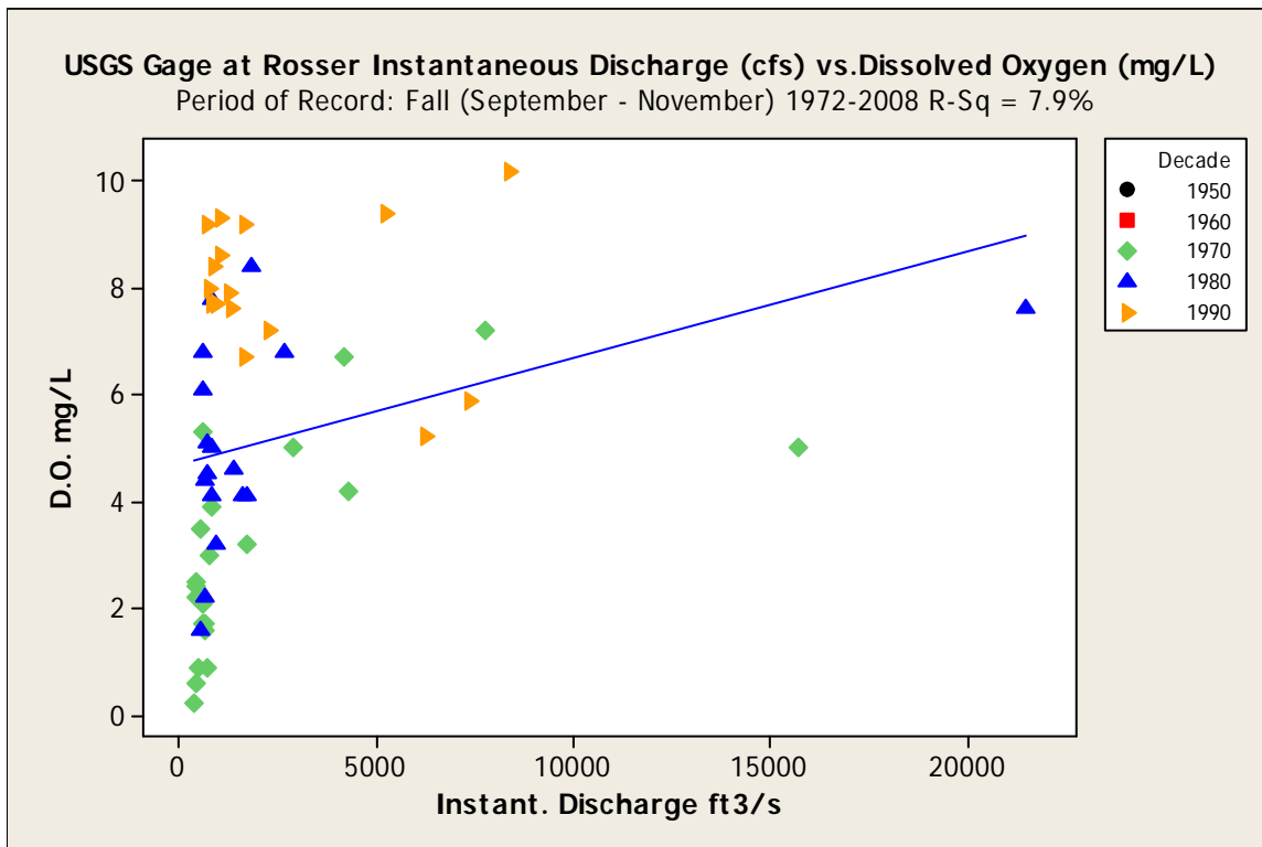
Figure 66. Flow versus fall dissolved oxygen at the Trinity River at Rosser 08062500 gage during 1972 through 2008.
