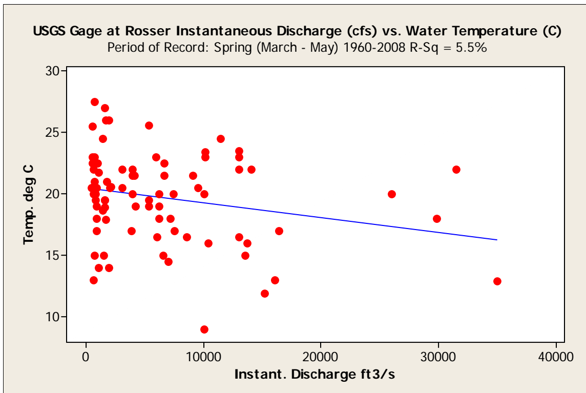
Figure 60. Flow versus spring water temperature at the Trinity River at Rosser 08062500 gage during 1959 through 2008.
