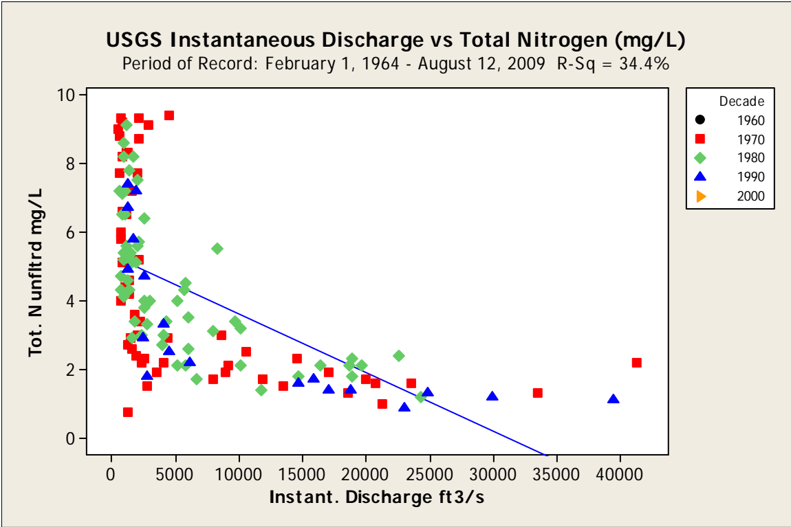
Figure 102. Flow versus total unfiltered nitrogen concentration at the Trinity River near Crockett 08065350 gage during 1972 through 2001. Matching flow and total nitrogen data lacking for 1960s and 2000s.
