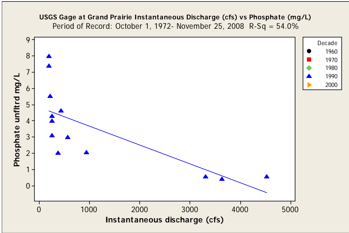
Figure 56. Flow versus total phosphate at the West Fork Trinity River at Grand Prairie 08049500 gage during 1972 through 2008. Matching flow and phosphate data only available for 1990s.
