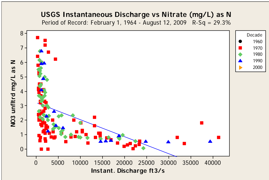
Figure 105. Flow versus nitrate as nitrogen concentration at the Trinity River near Crockett 08065350 gage during 1972 through 2001. Matching flow and nitrate nitrogen data lacking for 1960s and 2000s.
