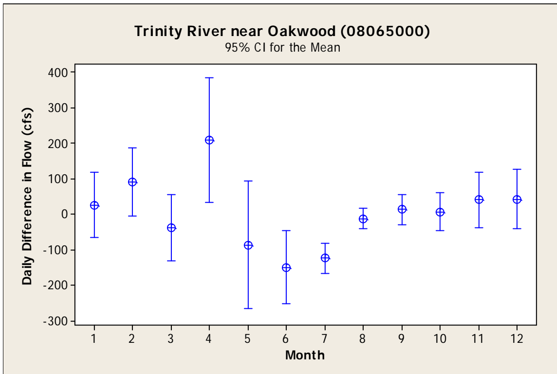
Figure 29. Monthly mean and 95% confidence intervals for daily difference in average daily flows between successive dates recorded at the USGS Trinity River at Oakwood (08065000) gage from 1924 through 2008.
