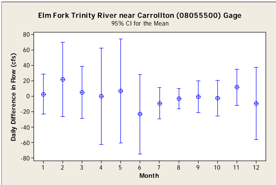
Figure 9. Monthly mean and 95% confidence intervals for daily difference in average daily flows between successive dates recorded at the Elm Fork Trinity River near Carrollton (08055500) gage from 1907 through 2008.
