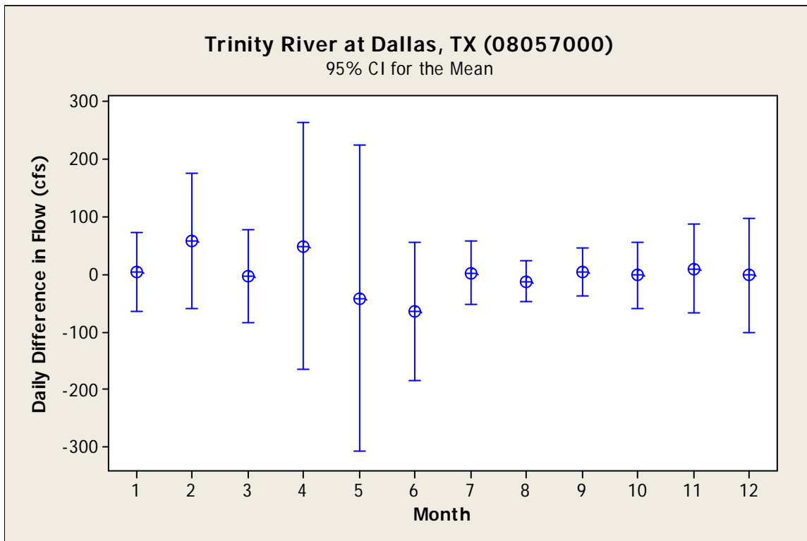
Figure 17. Monthly mean and 95% confidence intervals for daily difference in average daily flows between successive dates recorded at the USGS Trinity River at Dallas (08057000) gage from 1904 through 2008.
