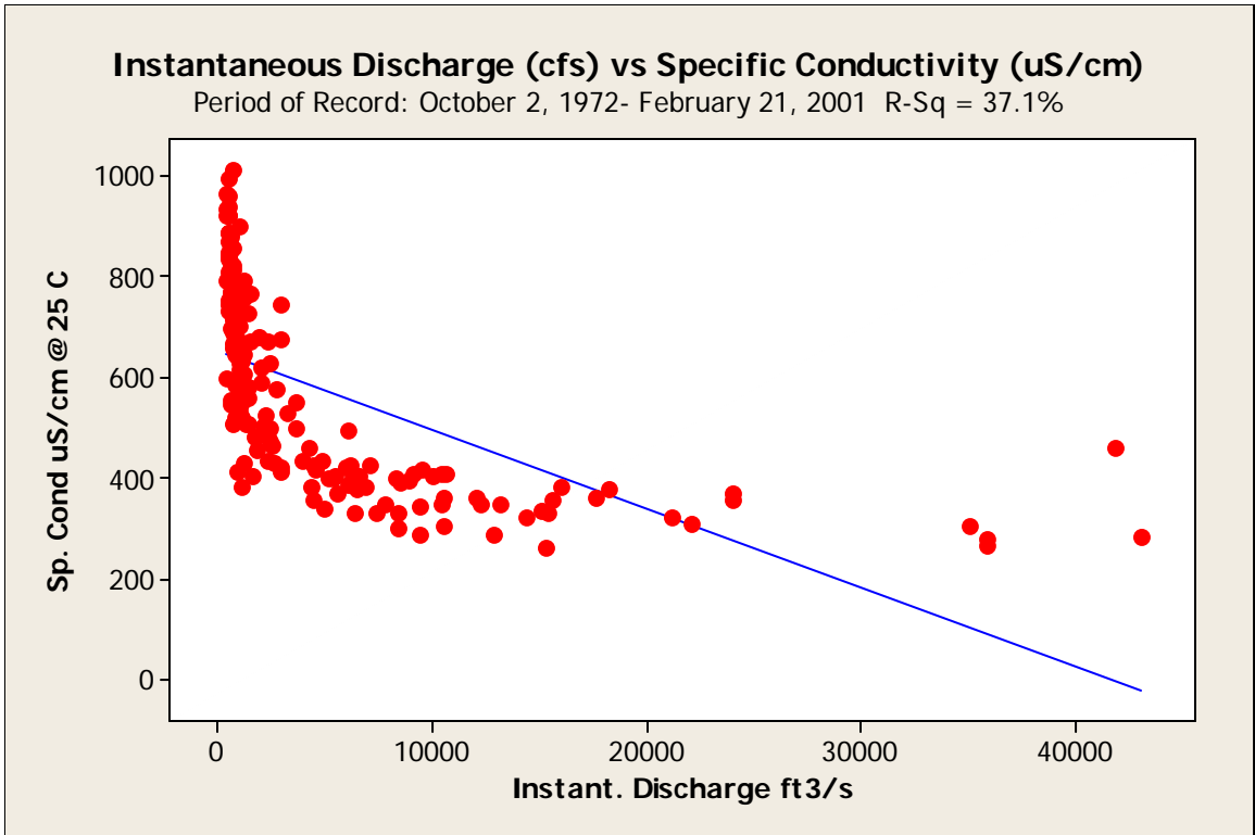
Figure 101. Flow versus specific conductance at the Trinity River near Crockett 08065350 gage during 1972 through 2001.
