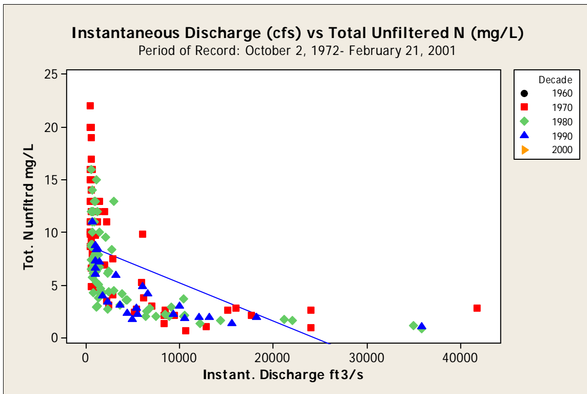
Figure 84. Flow versus total nitrogen unfiltered at the Trinity River at Trinidad 08062700 gage during 1972 through 2001. Matching flow and total nitrogen data lacking for 1960s and 2000s.
