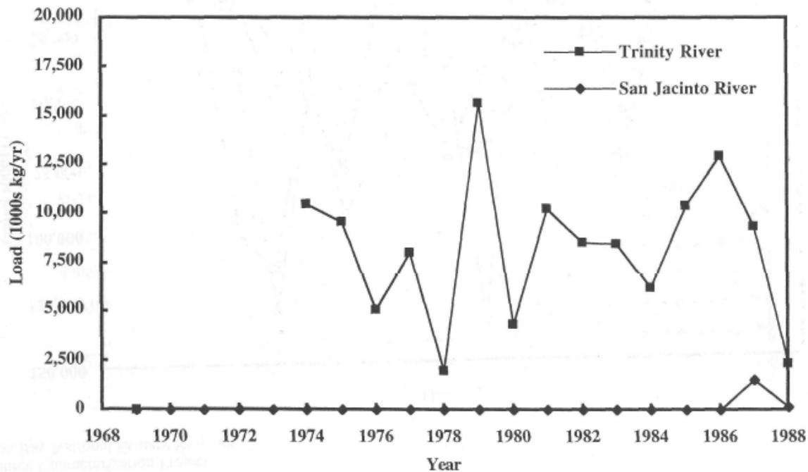
Figure 141. Estimated loads of total nitrogen into Galveston Bay from the Trinity River at Romayor and from the San Jacinto River from 1969 through 1988. Source: (Armstrong and Ward Jr. 1993)
