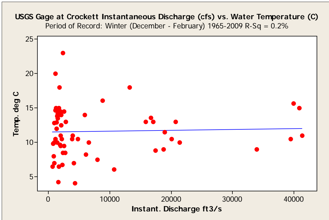
Figure 93. Flow versus winter water temperature at the Trinity River near Crockett 08065350 gage during 1965 through 2009.
