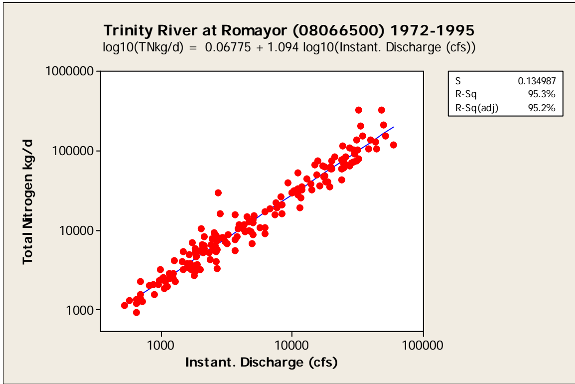
Figure 130. Flow versus total unfiltered nitrogen loading at the Trinity River at Romayor 08066500 gage based on the period of record 1972 through 1995.
