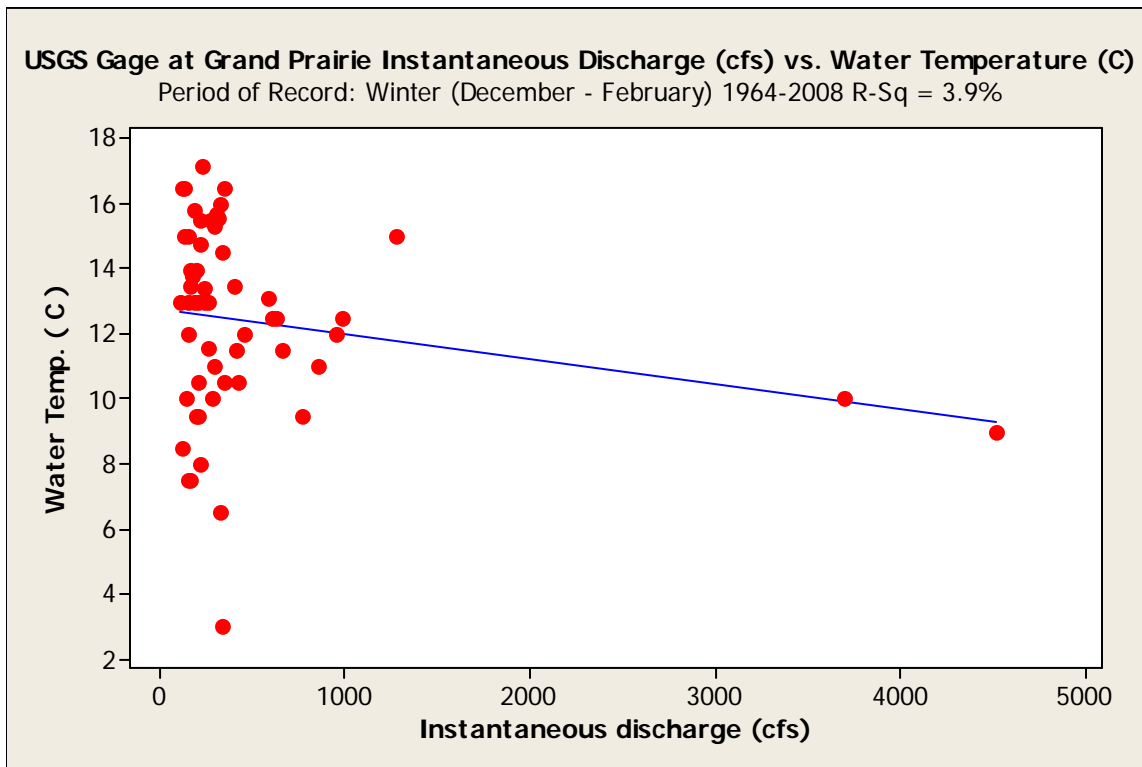
Figure 43. Flow versus winter water temperature at the West Fork Trinity River at Grand Prairie 08049500 gage during 1964 through 2008.
