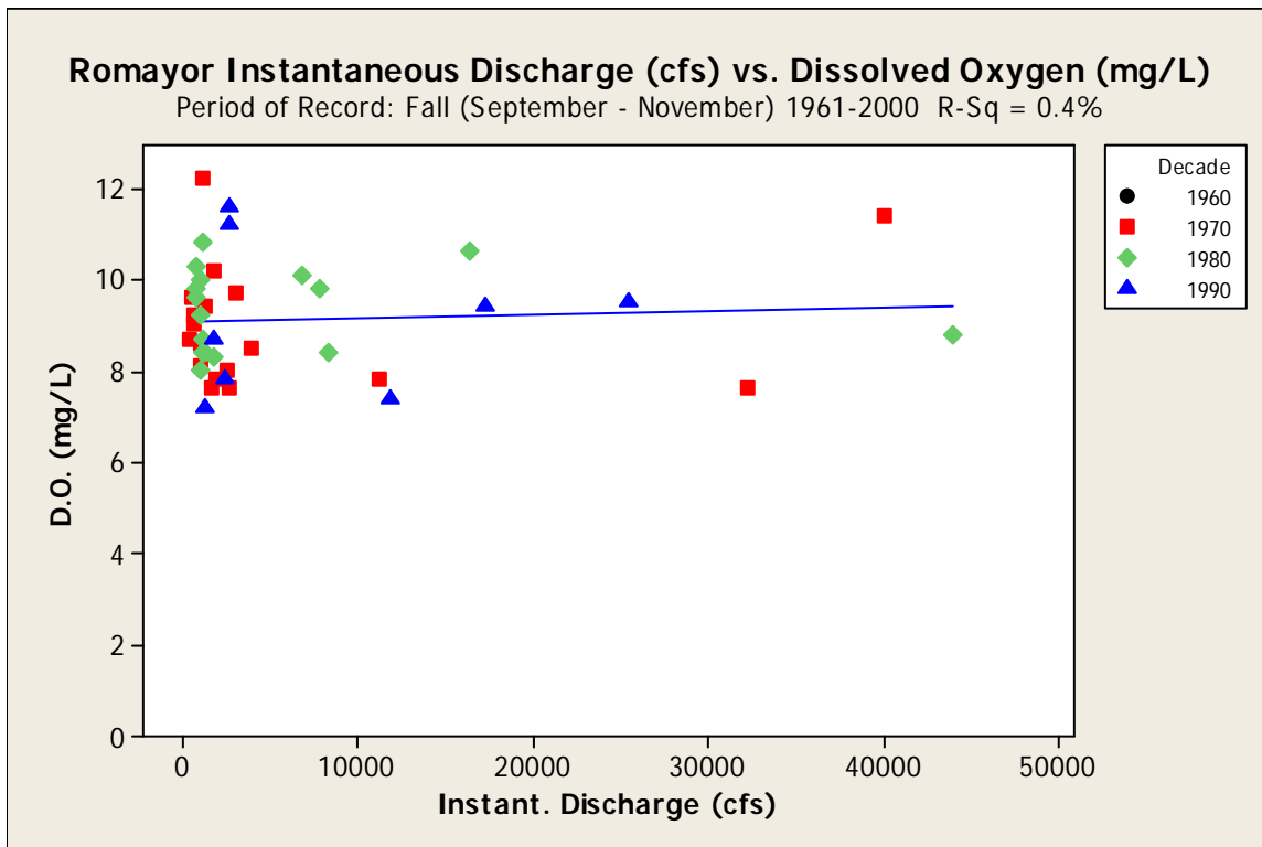
Figure 121. Flow versus fall dissolved oxygen at the Trinity River at Romayor 08066500 gage during 1961 through 2000. Matching flow and dissolved oxygen data lacking for 1960s and 2000s.
