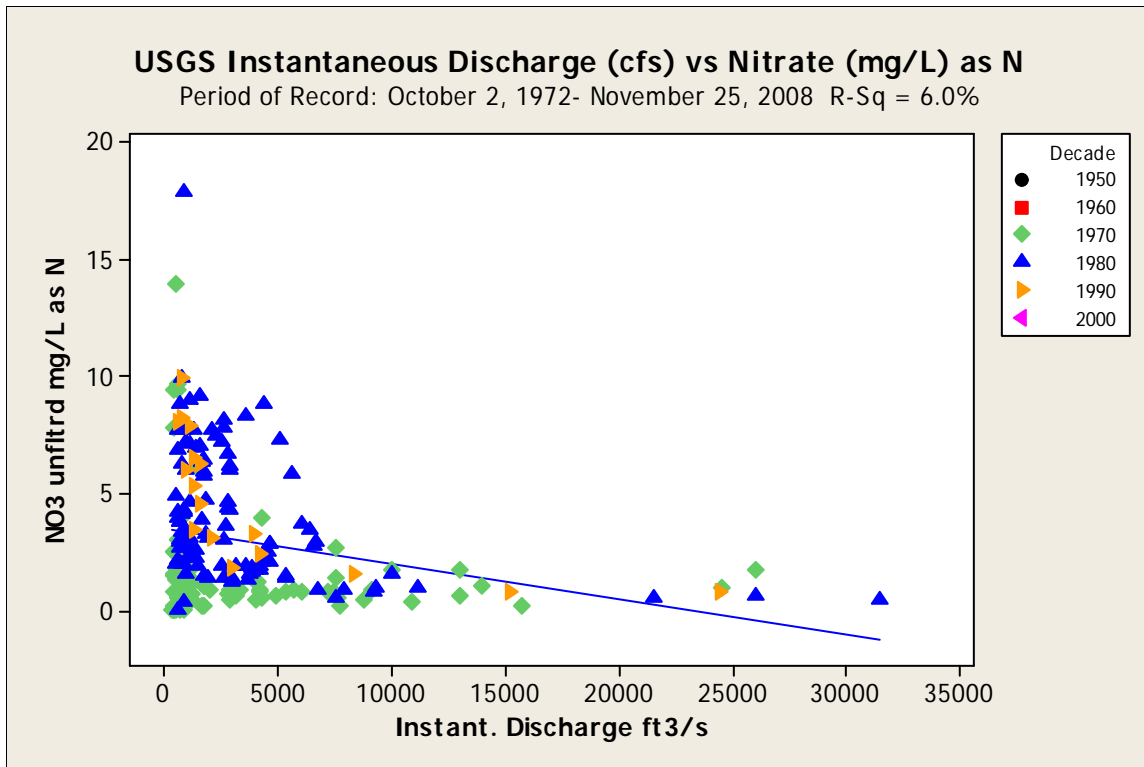
Figure 71. Flow versus nitrate as N unfiltered at the Trinity River at Rosser 08062500 gage during 1972 through 2008. Matching flow and nitrates + nitrites data lacking for 1950s, 1960s and 2000s.
