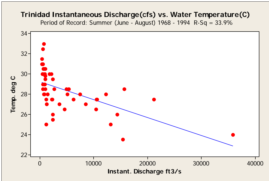
Figure 77. Flow versus summer water temperature at the Trinity River at Trinidad 08062700 gage during 1966 through 1994.
