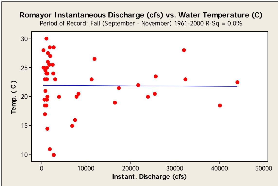
Figure 117. Flow versus fall water temperature at the Trinity River at Romayor 08066500 gage during 1961 through 2000.
